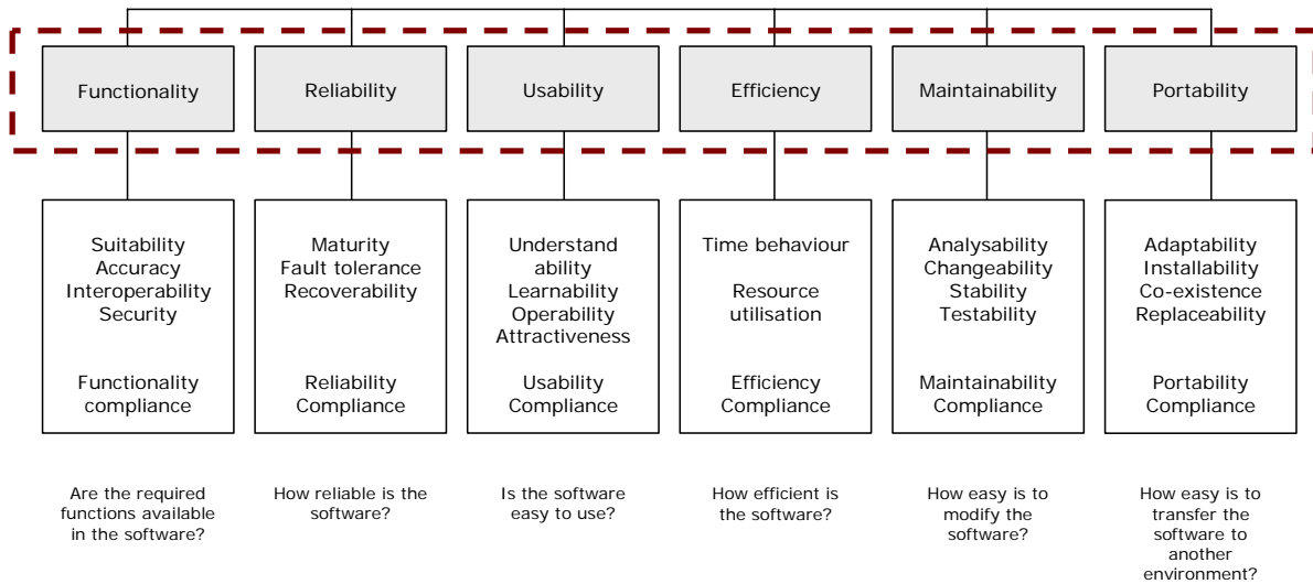
Fig. 12 ISO-IEC 9126 quality model
