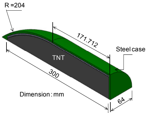
Fig. 1 Shape and dimension of a dummy warhead
