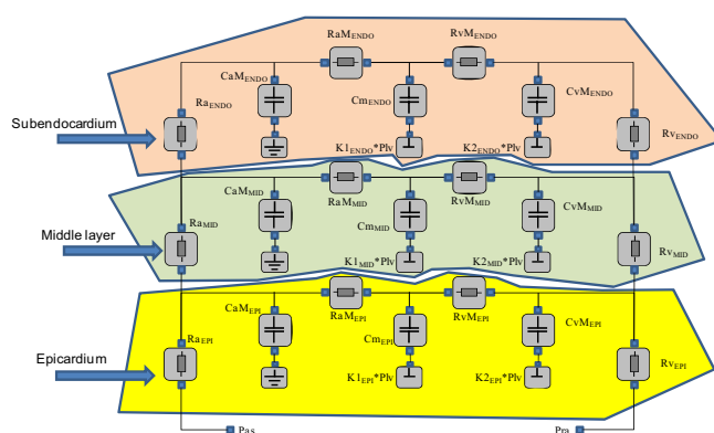
Fig. 2 Electric analogue of the coronary circulation. Three parallel vascular sections reproduce the subendocardial, the middle and the subepicardial layers of the left ventricular wall. Ra_i is arterial resistance; RaM_i ( CaM_i ) is the arteriolar resistance (compliance); Cm_i is the capillary compliance; RvM_i ( CvM_i ) is the venular resistance (compliance); Rv_i is the venous resistance. (i= EPI, MID, ENDO.)
