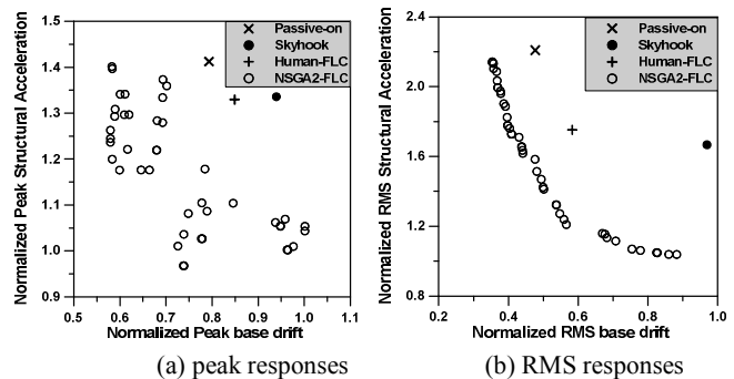
Fig. 9 Optimization results with two RMS objectives
