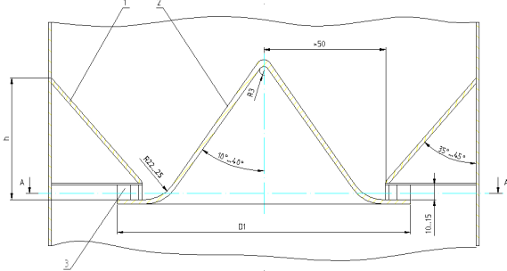
Fig. 10 Constructive design of the grid
