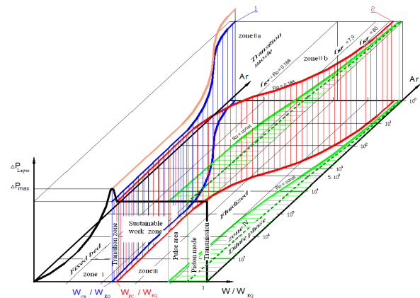
Fig. 9 Working regions of fluidized systems
