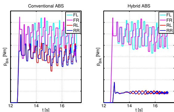
Fig. 7 Brake pressures
