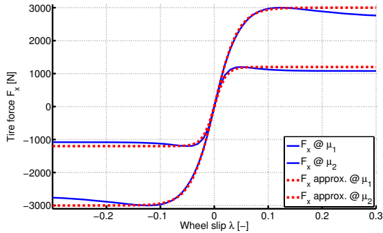
Fig. 3 Tire force approximation
