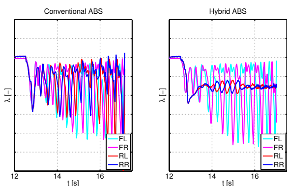
Fig. 9 Wheel slips
