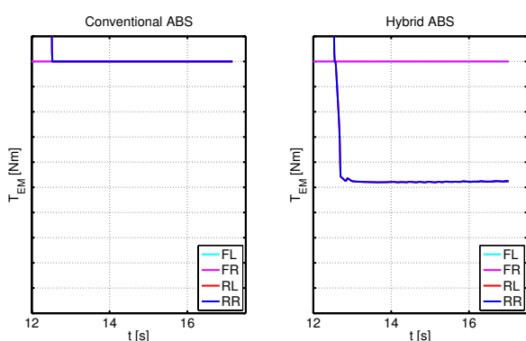
Fig. 8 Traction motor torques
