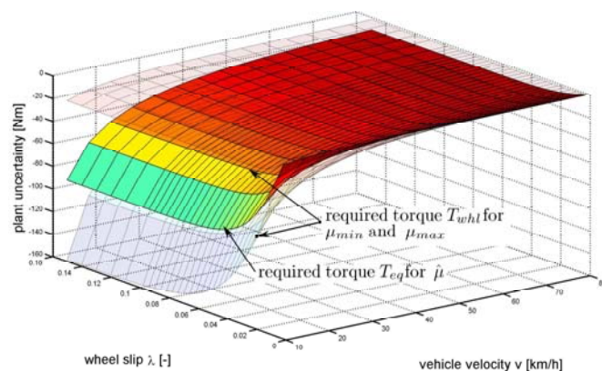
Fig. 5: Model Uncertainties
