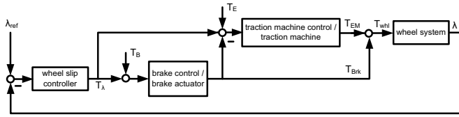
Fig. 4 Control loop
