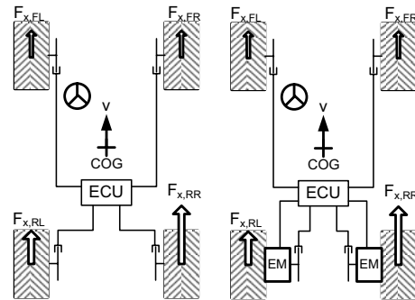
Fig. 1 Vehicle topology
