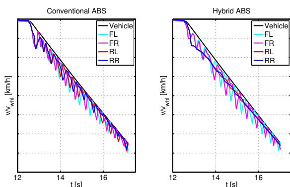
Fig. 10 Wheel velocities
