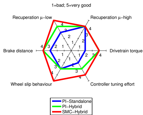
Fig. 6 Controller rating
