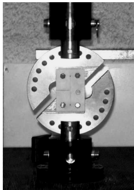
Fig. 4 Geometry of the loading and modified version of Arcan specimen
