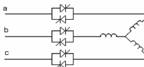
Fig. 1: The model of induction motor-AC converter.
