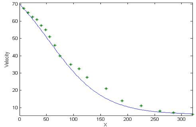
Fig. 4 Measured mean axial velocity along flame centre line in radial direction (points) for combustion [15] against the analytical solution (solid line)
