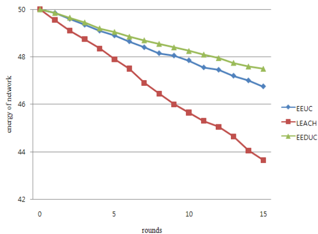
Fig. 5 The total remaining energy of the network
