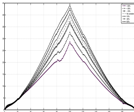
Fig. 10. Correlation plot of predicted primary energy values with variation of \pm 50\% with ideal input
