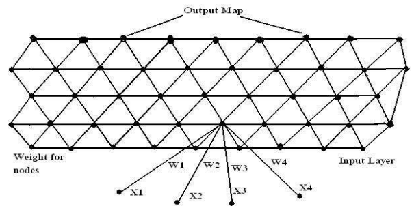
Fig. 3. Self Organizing Feature Map
