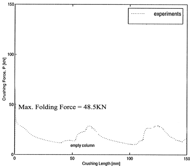
Fig. 7 Experimental folding force versus axial displacement in a square column (80mm×80mm) [17]
