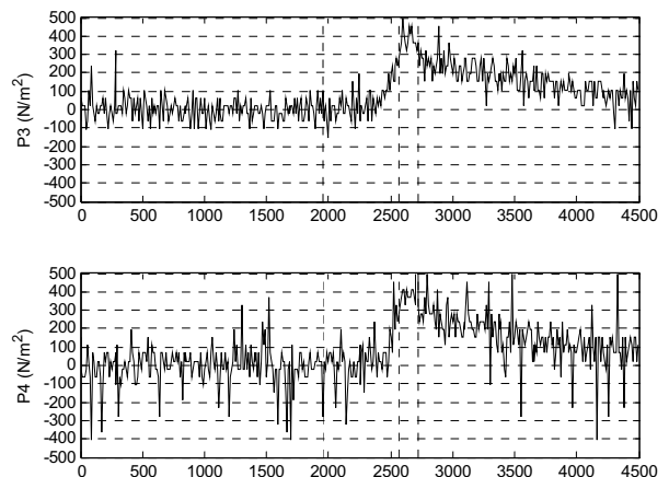
Fig. 14. Gage pressures at P3 and P4 vs. time for the 7.125"-diameter capsule with air valves completely opened.
