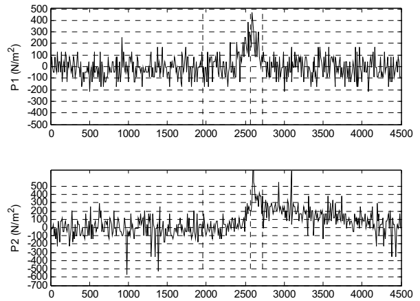
Fig. 13. Gage pressures at P1 and P2 vs. time for the 7.125"-diameter capsule with air valves completely opened.
