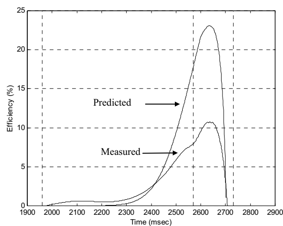
Fig. 18. The measured and predicted TLIM efficiency vs. time for the 7.125"-diameter capsule with air valves completely opened.
