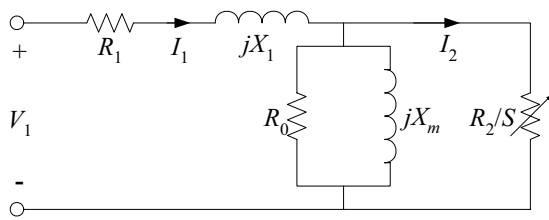
Fig. 2. The modified per-phase TLIM equivalent circuit with a capsule inside the entire TLIM stator.
