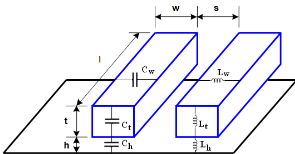
Fig. 5 Interconnect modelling of the substrate
