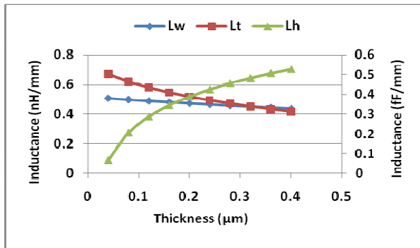
Fig. 8 Simulation results of interconnect Inductance for the proposed adder
