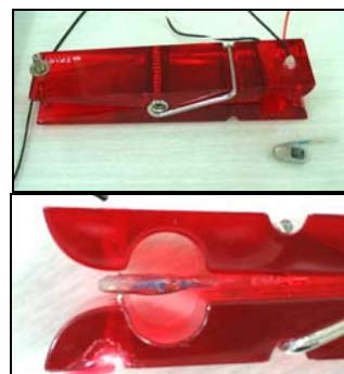
Fig. 3 Data receiver
