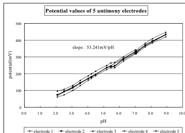
Fig. 6 Potential values of 5 antimony electrodes
