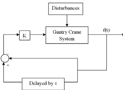
Fig. 2 Delayed feedback signal controller structure
