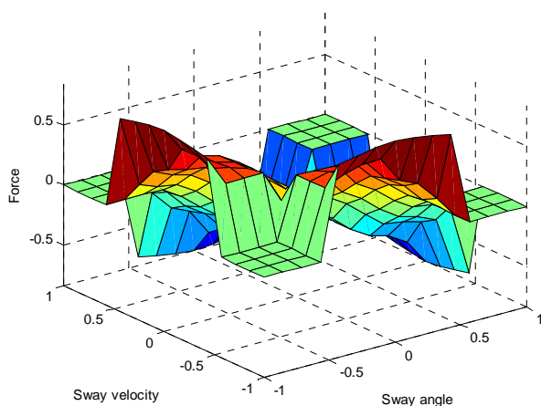
Fig. 4 Control surface of the Fuzzy Logic Controller
