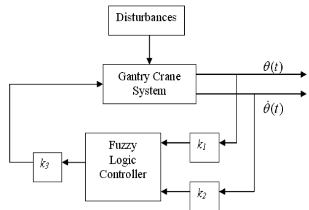
Fig. 3 PD-type Fuzzy Logic Controller structure
