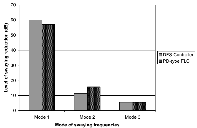
Fig. 9 Level of swaying angle reduction using DFS and PD-type Fuzzy Logic Controller
