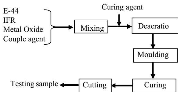
Fig. 1 The schematic procedure of sample preparation
