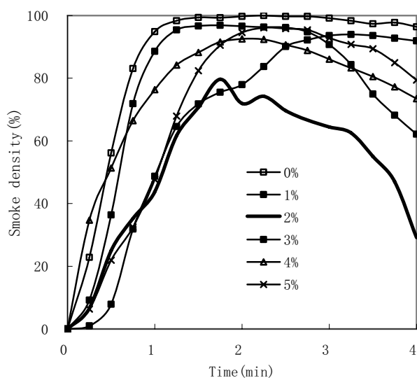
Fig. 3 The effect of copper oxide content on the smoke density of EP/IFR/Titanate system b The addition content of copper oxide is based on epoxy resin mass
