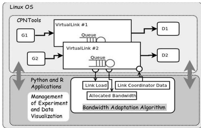
Fig. 2 Simulation scheme using CPN Tools
