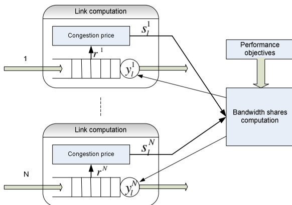
Fig. 1 Bandwidth shares computation scheme
