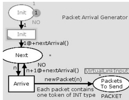
Fig. 4 Traffic simulation using CPN Tools
