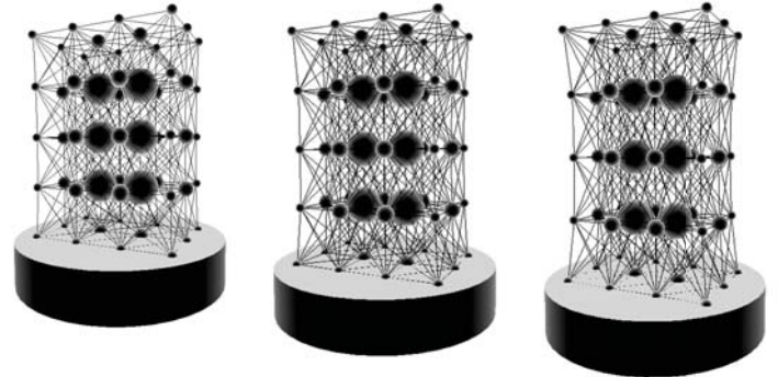
Fig. 3. Optimized MSM with different loads
