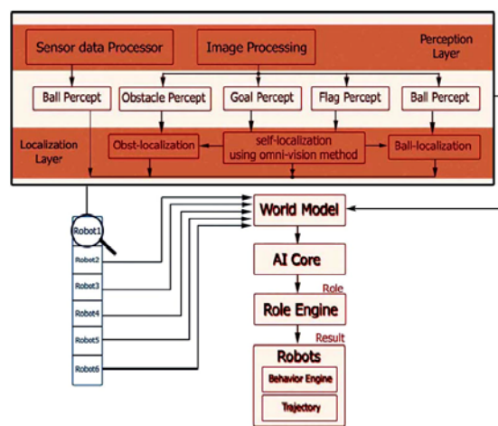
Fig. 10 World model construction and artificial intelligent structure
