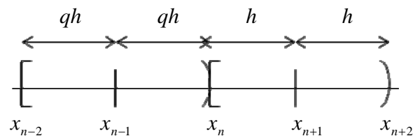
Fig. 1 2-point block method of variable step size
