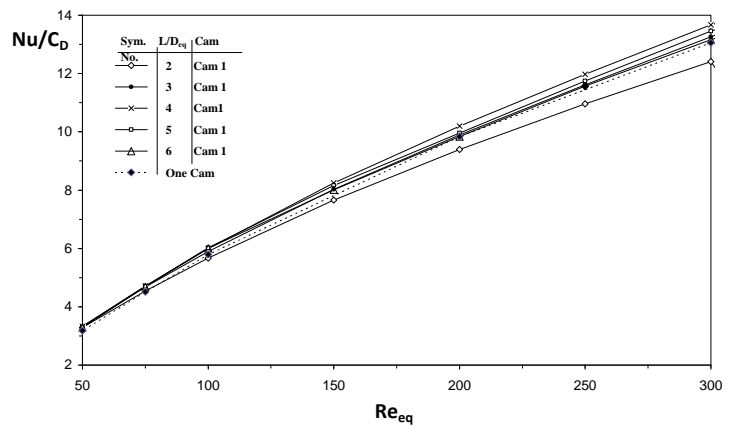
Fig. 7 Variation of \rho f Nu/C with Reynolds number and longitudinal pitch ratio
