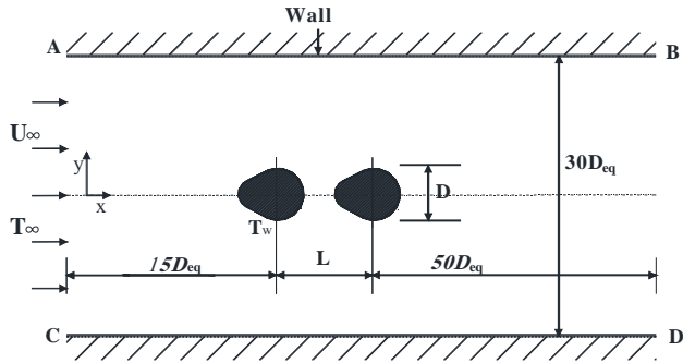
Fig. 2 Solution Domain
