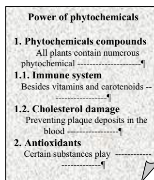
Fig. 1 Textual document
