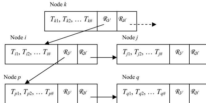
Fig. 4 Model implementation
