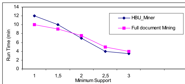
Fig. 5.b. Runtime comparison between full document mining and hierarchical mining for document 2.
