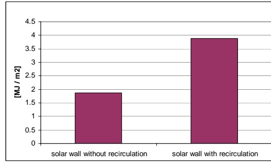
Fig. 27 Daily solar heat gain
