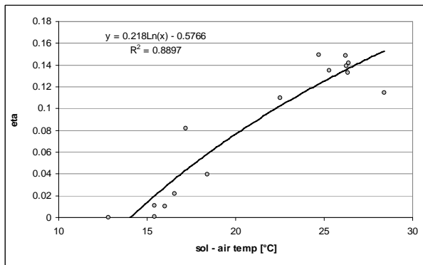
Fig. 26 Yield and sol – air temperature
