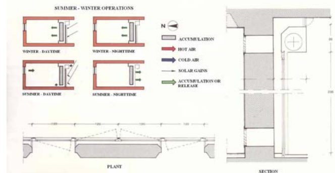
Fig. 8 Management of solar wall
