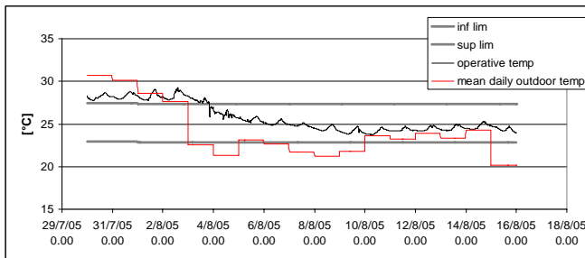
Fig. 15 Indoor ASHRAE comfort
