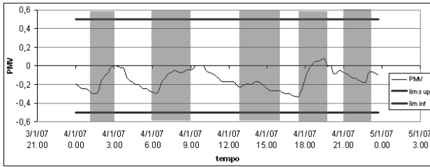
Fig. 9 Daily PMV and operation schedule
