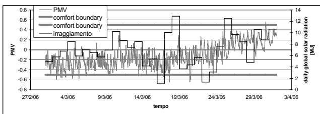
Fig. 11 PMV and global solar radiation in March
