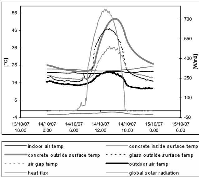
Fig. 19 Monitored value on October the 14, 2007
