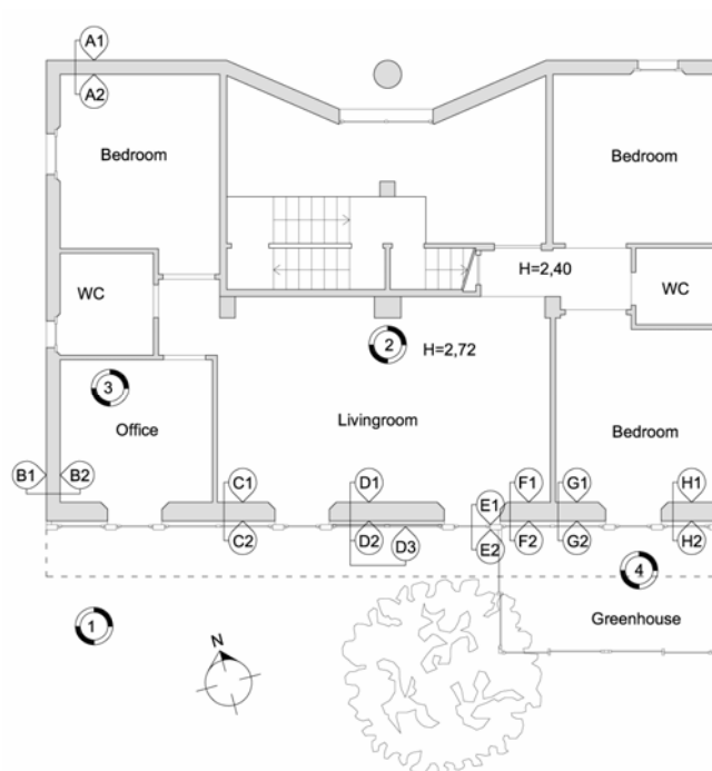
Fig. 2 Position of probes and monitoring station
