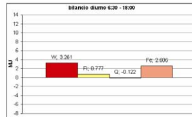
Fig. 22 Day 2 cloudy (daytime)
