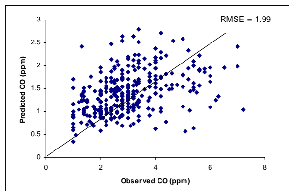
Fig. 3 Observed Vs Predicted CO (IITLS)
