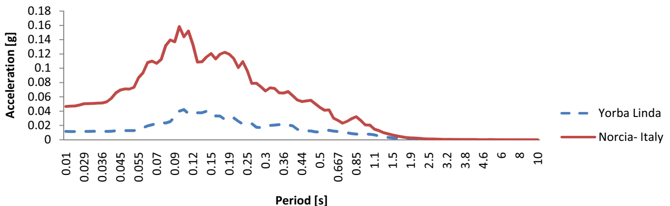
Fig. 6 Spectral acceleration of Yorba Linda and Norcia-Italy horizontal records from PEER
