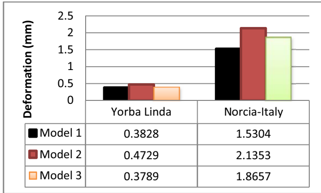
Fig. 11 Maximum directional deformation under 'empty' condition
