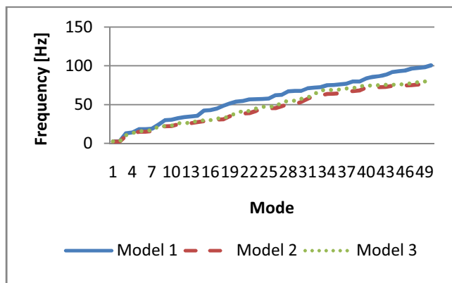
Fig. 8 Frequencies of the first 50 modes under 'full' condition
