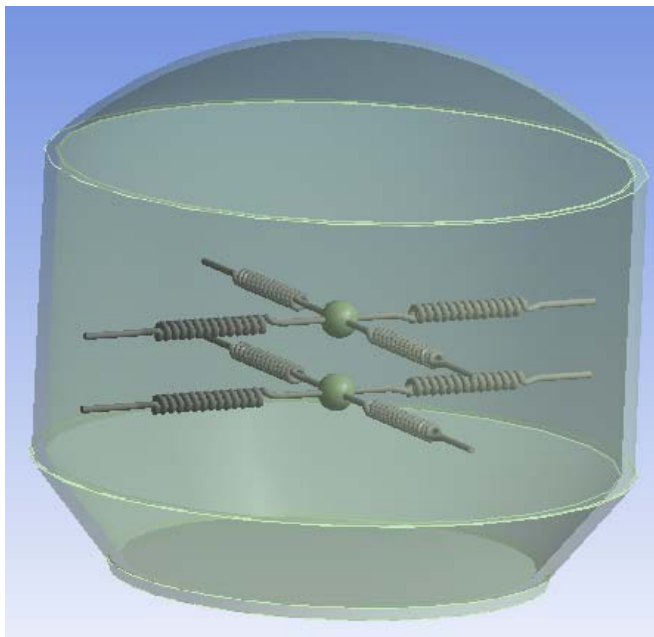
Fig 4 Two degree of freedom spring-system
