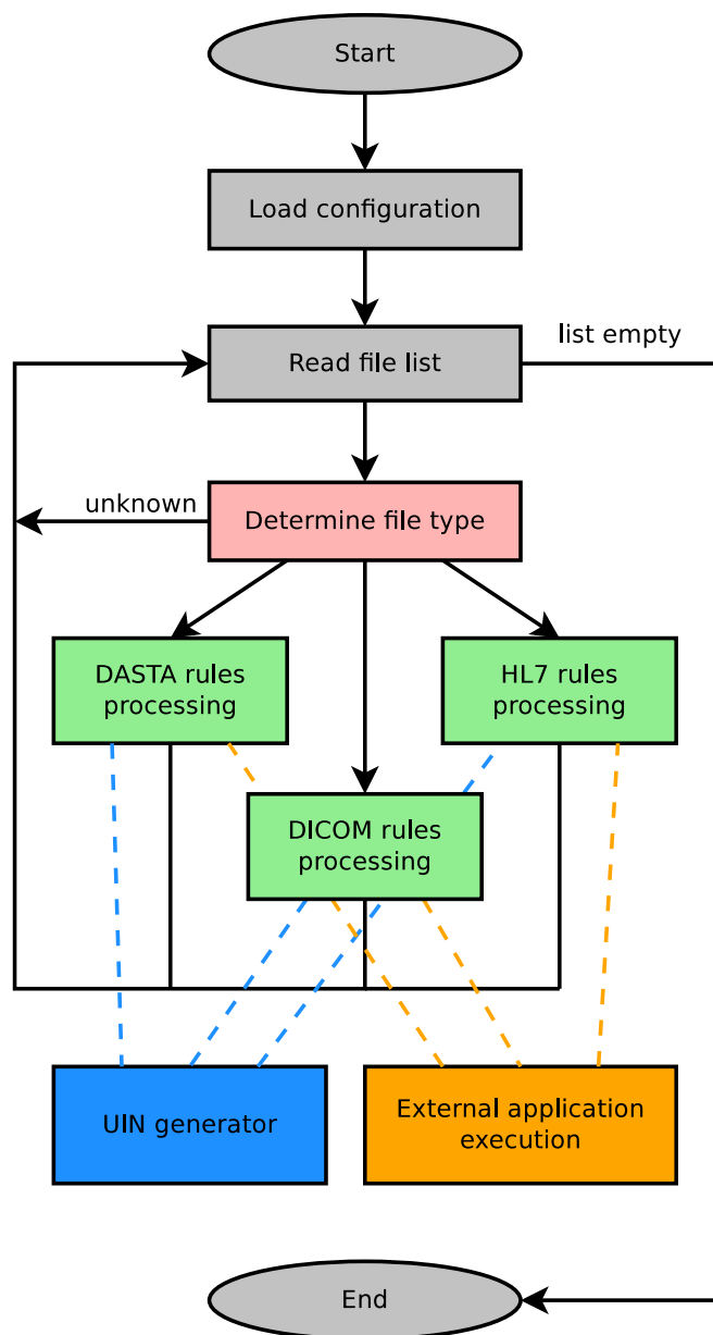
Figure 2. The de-identification AnonMed application flow chart.
