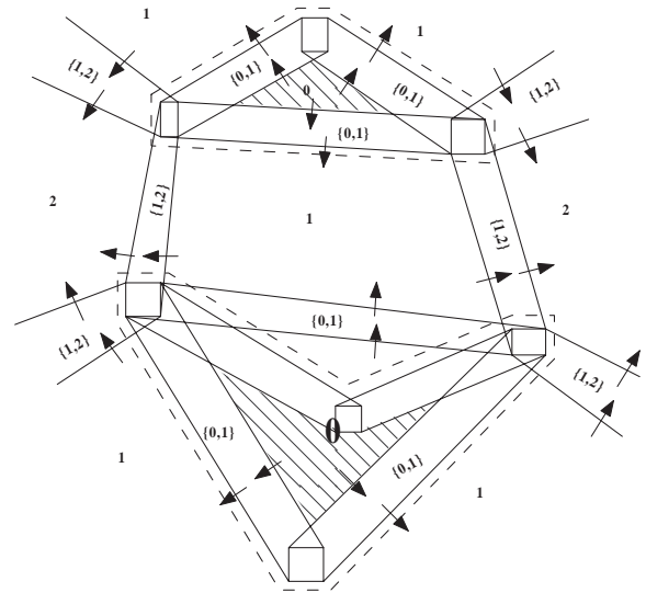
Fig. 8: A partial visual number partition of \mathbb{R}^2
