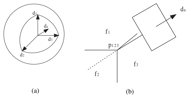
Fig. 5: (a) a unite sphere and 3 plane normals d_1, d_2 and d_3 ; (b) p_{123} being the furthest point along d_a ;
