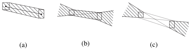
Fig. 3: (a) a partial line segment (PLS) (b) a partial line (PL) (c) two partial half lines (PHL)
