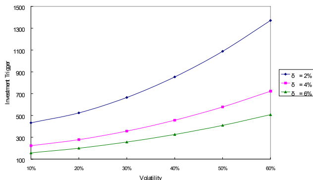
Fig. 1. The Variance Effect under a GBM
