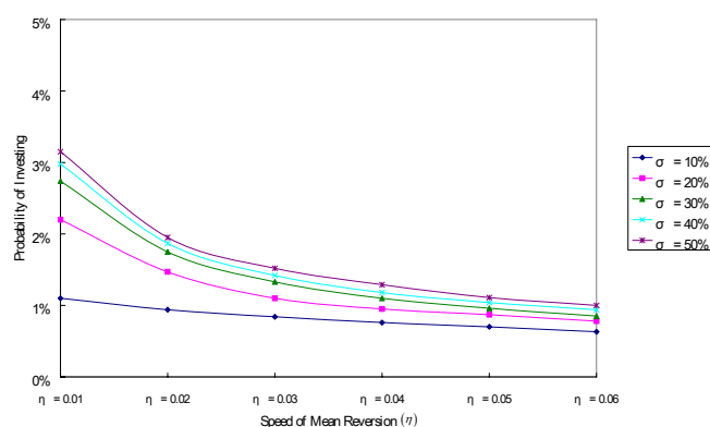
Fig. 7. The Probability of Investing under a Mean-Reverting Process as a Function of Mean-Reverting Speed ( \eta )
