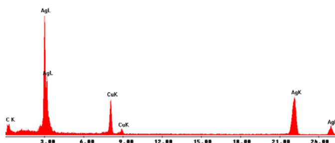
Fig.4.- Energy-dispersive spectroscopy spectrum of silver nanoparticles prepared from 1.1 mM AgNO 3 solution.
