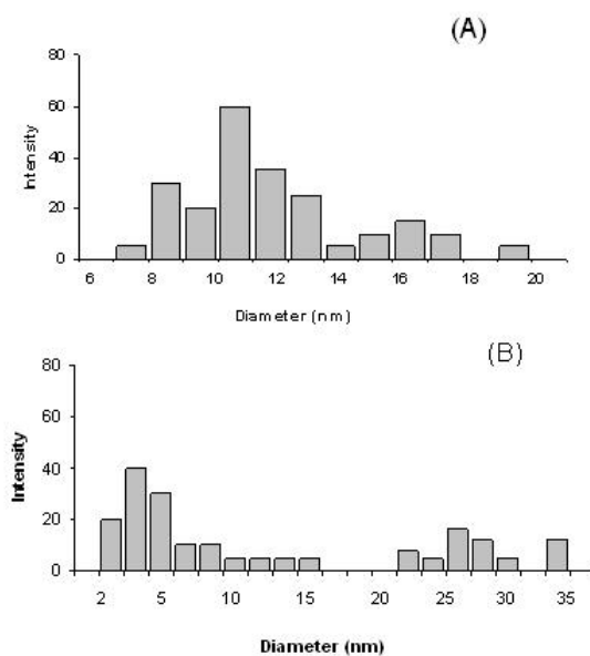
Fig.10.- Particle size distributions of Ag nanoparticles (prepared from 1.1 mM AgNO 3 solution) and citrate of sodium solution with a concentrate ranging from 1.0 mM (A) to 2.0 mM (B).
