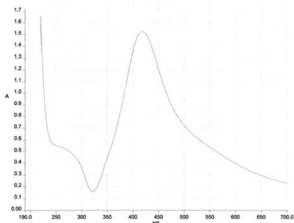
Fig. 2.-UV-Vis absorption spectrum of silver nanoparticles obtained.
