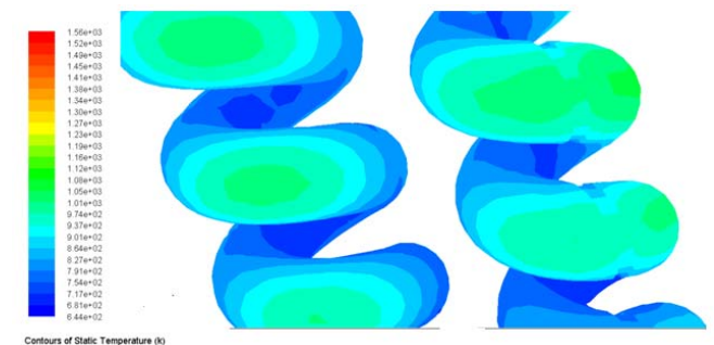
Fig. 9 Contours of static temperature for cooling ducts having turbulators of e/D = 0.04 and 0.75mm rib thickness
