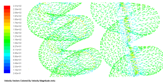
Fig. 24 Velocity vectors for cooling ducts having turbulators of e/D = 0.08 and 0.5\text{mm} rib thickness
