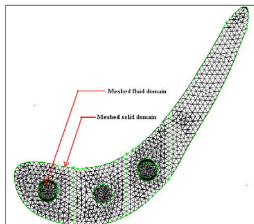
Fig. 2 Gas turbine blade modeled in CATIA and meshed in GAMBIT
