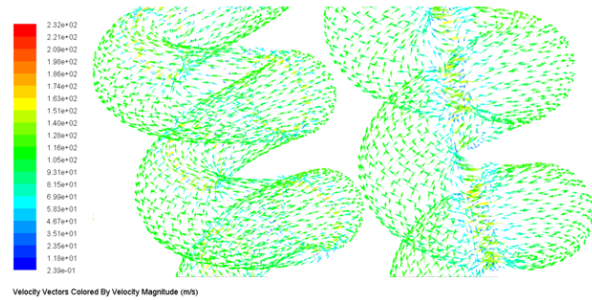
Fig. 25 Velocity vectors for cooling ducts having turbulators of e/D = 0.08 and 0.75\text{mm} rib thickness
