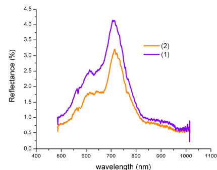
Fig. 3 Diffuse reflectance spectra of contaminated wound after laser irradiation (wound no. 4 / pig no.1); (1) – before laser irradiation; (2) – after laser irradiation
