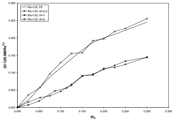
Fig. 3 Normalized fractal dimension of heavy particle lines as a function of the normalized time for k_N/k_1=36 and different particle drift velocities
