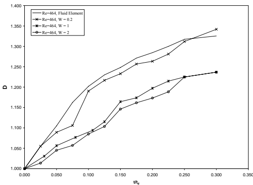
Fig. 4 Fractal dimension of heavy particle lines as a function of the normalized time for k_N/k_1=100 and different particle drift velocities
