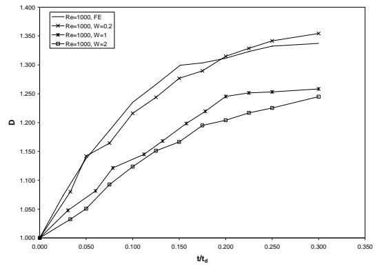
Fig. 6 Fractal dimension of heavy particle lines as a function of the normalized time for k_N/k_1=178 and different particle drift velocities
