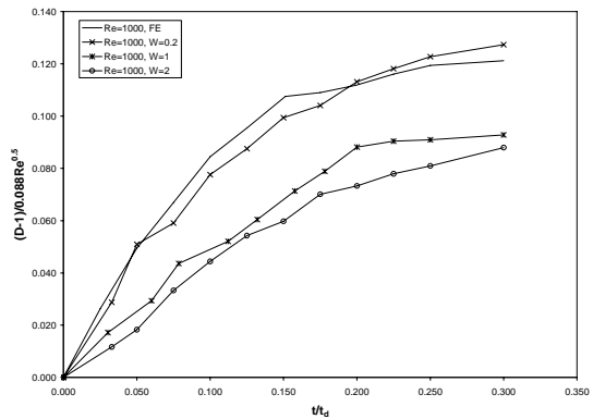
Fig. 7 Normalized fractal dimension of heavy particle lines as a function of the normalized time for k_N/k_1=178 and different particle drift velocities
