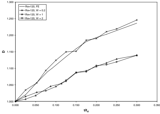
Fig. 2 Fractal dimension of heavy particle lines as a function of the normalized for k_N/k_1=36 and different particle drift velocities
