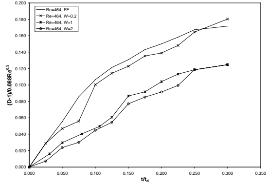
Fig. 5 Normalized fractal dimension of heavy particle lines as a function of the normalized time for k_N/k_1=100 and different particle drift velocities
