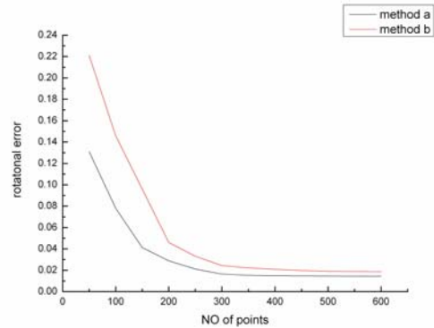
Fig. 6. Rotation error for Optimization for sampling strategy in freeform surface inspection
