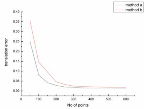
Fig. 5. Translation error for Optimization for sampling strategy in freeform surface inspection
