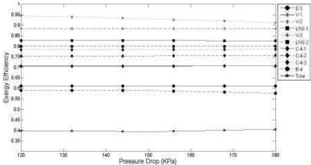
Fig. 7. Variation of Exergy Efficiency in each component with the change in V-3 pressure drop.
