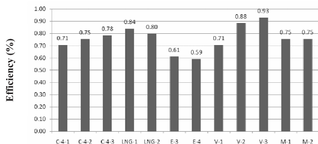
Fig. 3. Exergetic efficiencies of refrigeration cycle components.
