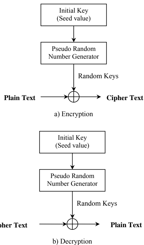
Fig. 1 Stream cipher
