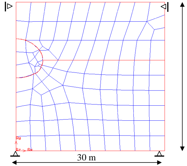
Fig. 5 Finite element mesh used in numerical simulation
