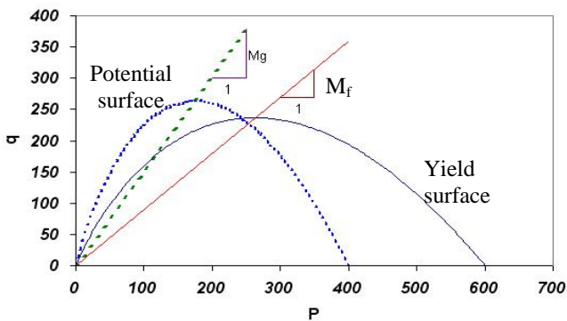
Fig. 1 Schematic yield and potential surfaces [13]
