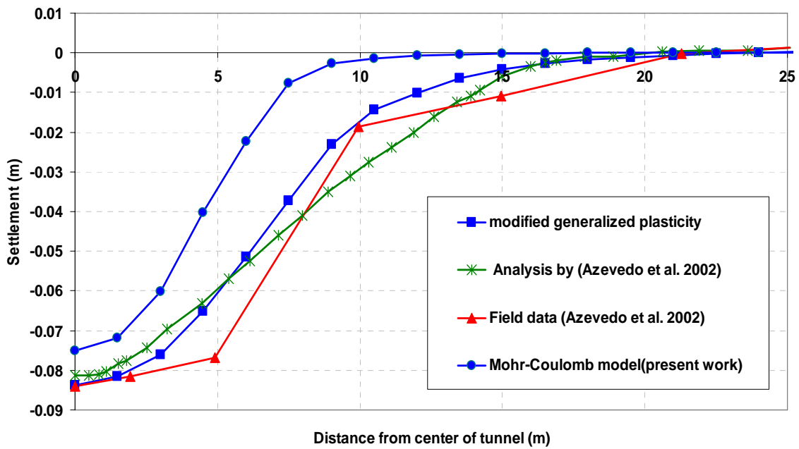
Fig. 6 Comparisons of predicted surface settlement profile and observed results
