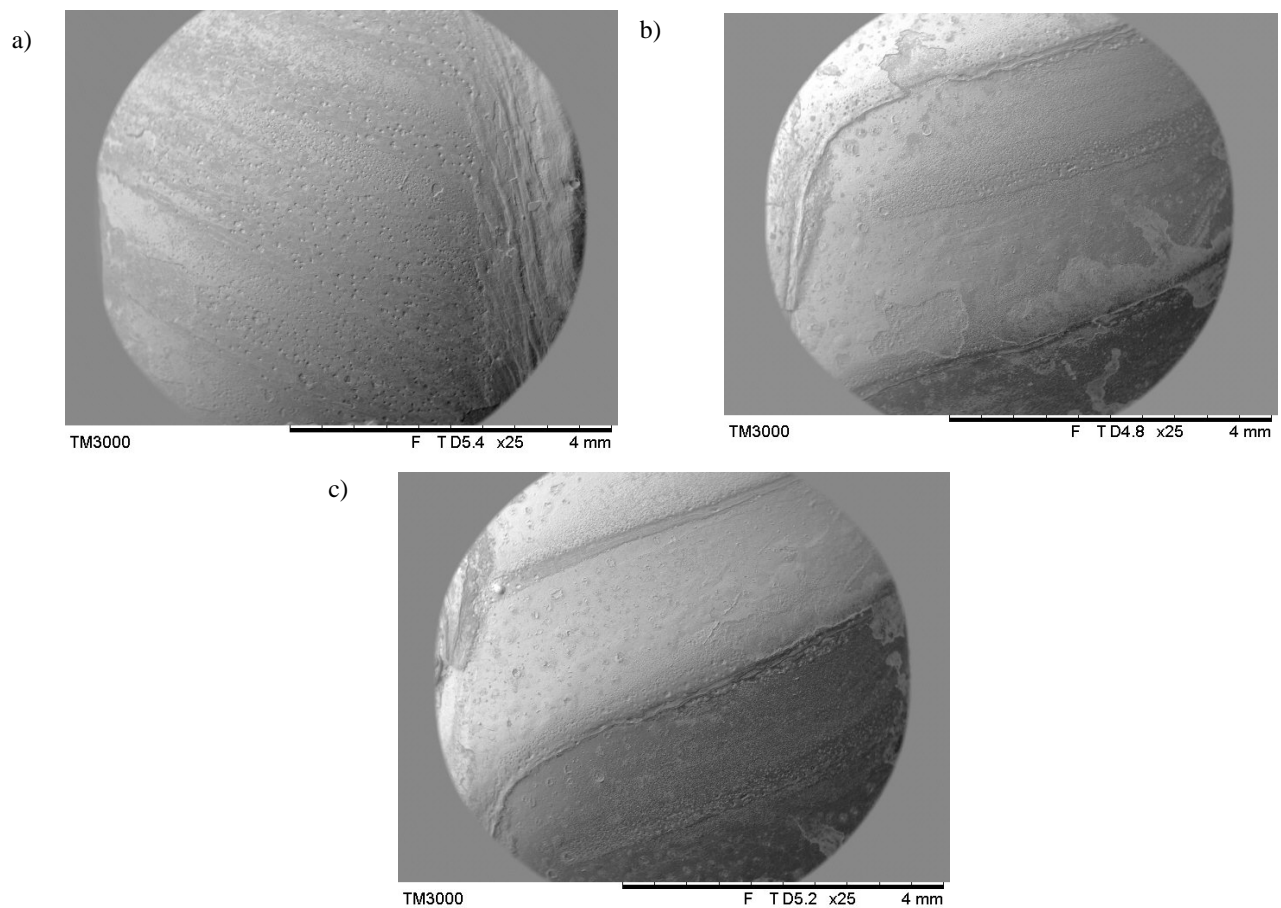
a) MRR = 5500-6400 \text{ mm}^3/\text{min} , SR = 20-30 \text{ } \mu\text{m} b) MRR = 3600-4800 \text{ mm}^3/\text{min} , SR = 30-50 \text{ } \mu\text{m} c) MRR = 3000-3500 \text{ mm}^3/\text{min} , SR = 65-80 \text{ } \mu\text{m}
