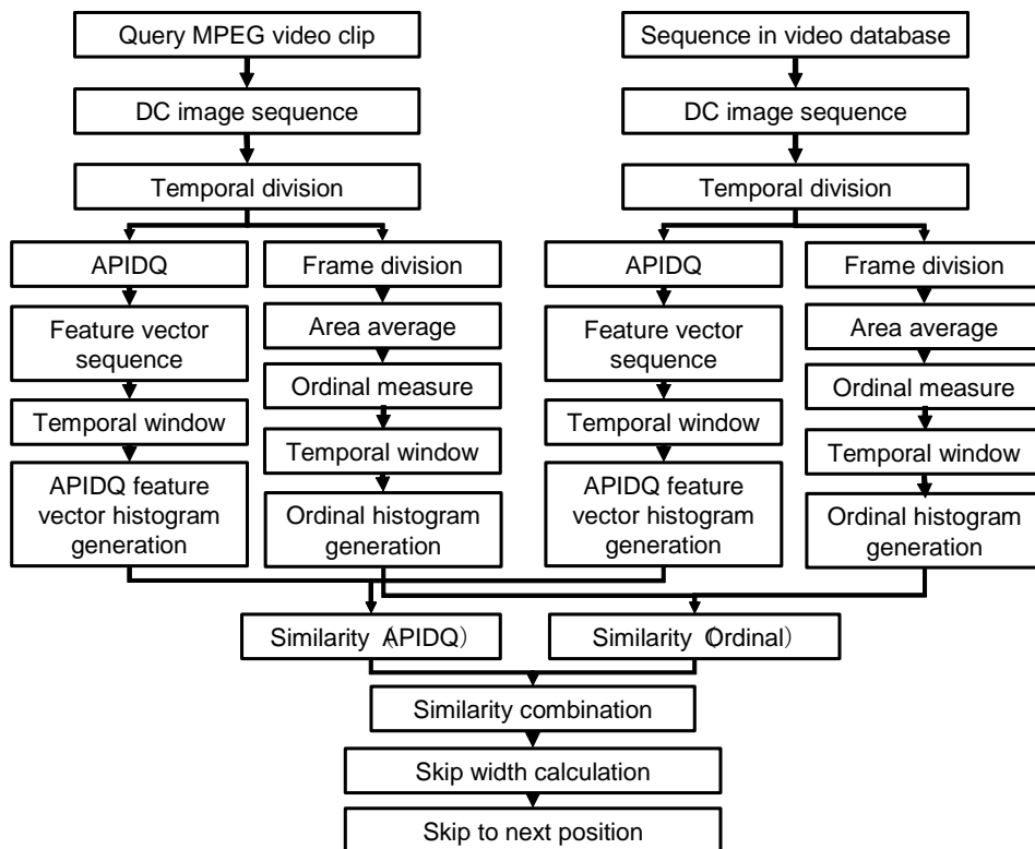
Fig.2 Proposed fast search algorithm.
