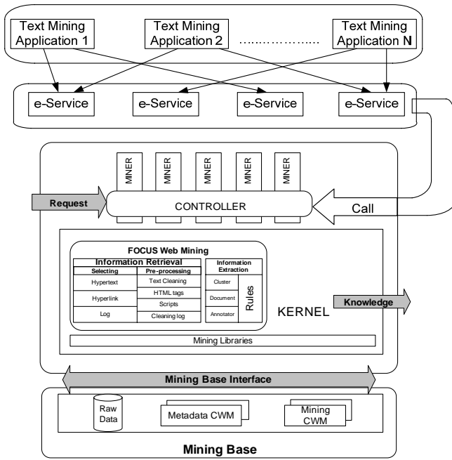
Fig. 5 The Flexible Web Text Mining Architecture
