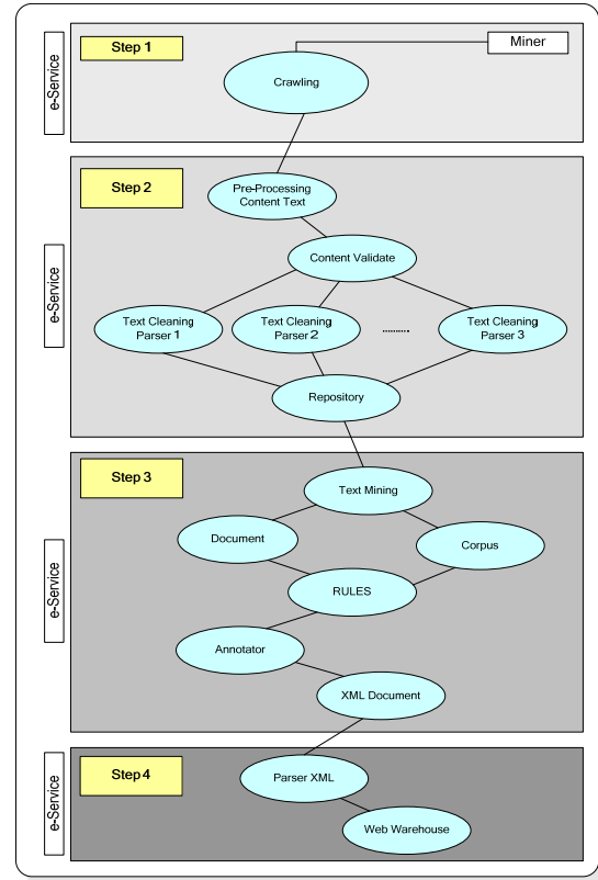
Fig. 6 E-service Workflow in Web Text Mining Process
