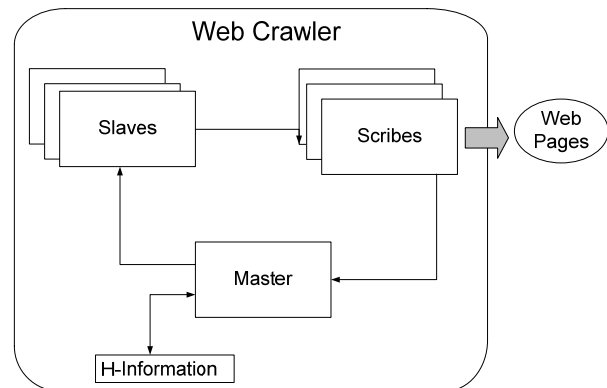
Fig. 3 Web Crawler Architecture
