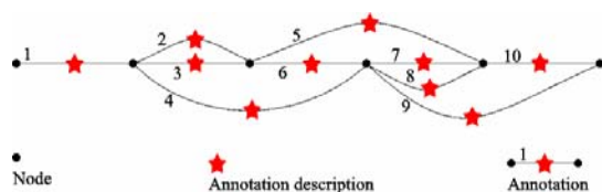
Fig. 4 Rules and Annotators scheme
