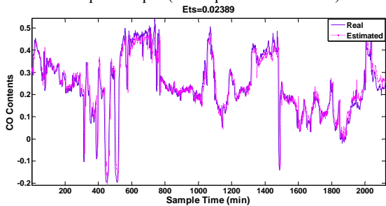
Fig. 11 Comparing between Prediction model and Real data for CO content output (5 min prediction horizon)
