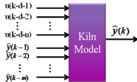
Fig. 6 Structure of simulation model
