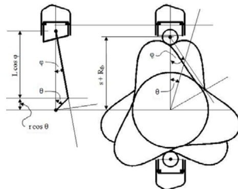
Fig. 2 conventional and Revetec engines
