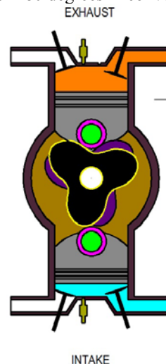
Fig. 1 Revetec engine with two cylinders
