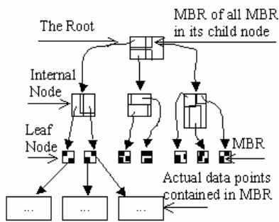
Fig. 5 Sample R*-tree
