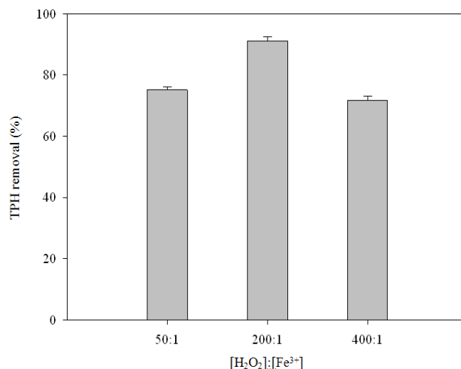
Fig. 1 Effect of [H_2O_2]:[Fe^{3+}] on TPH mass removal. Reported values are the mean one standard deviation ( n = 3 )
