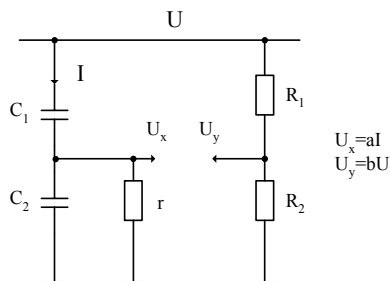
C_1, C_2 - bushing or CT under test R_1, R_2 - high voltage resistive divider (capacitive divider or voltage transformer) r - additional shunt resistor r \ll XC_2 After calibration \phi[U_x, U_y] \sim k \tan \delta
