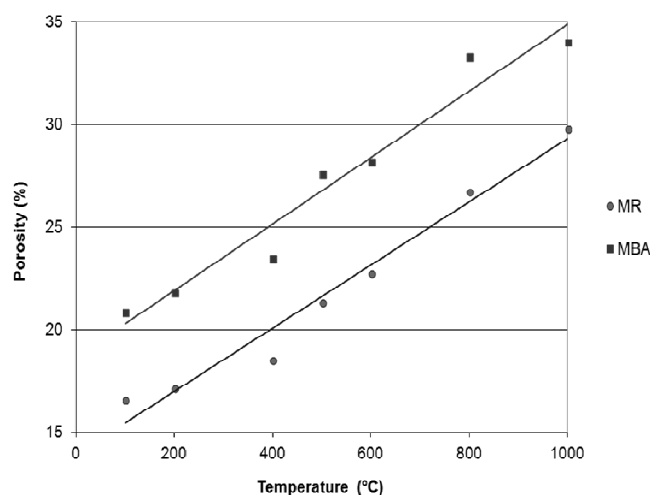
Fig. 5 Open porosity of mortars after temperature exposure
