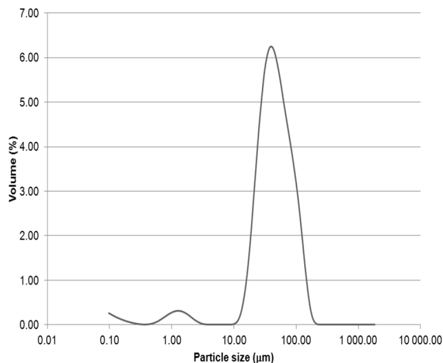
Fig. 3 Typical particle size distribution of powder sample
