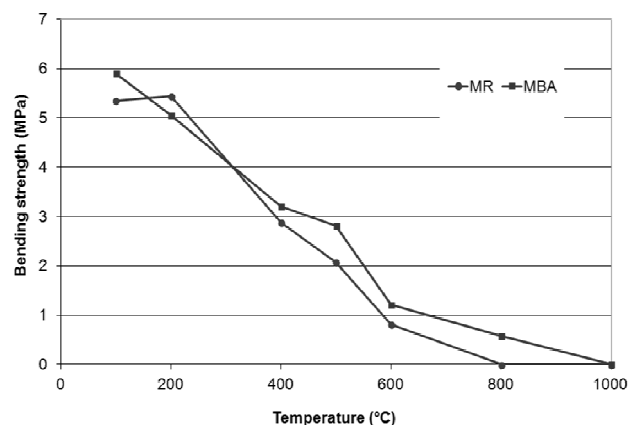
Fig. 7 Bending strength of mortars in dependence on temperature of exposure
