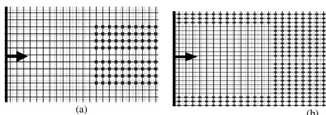
Fig. 9 (a) Coupling directly into PhC waveguide (no taper), (b) coupling through butt-coupled taper
