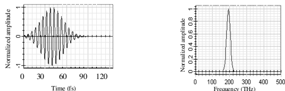
Fig. 8 The Gaussian-modulated CW signal and its spectrum, that is used as the input to the PhC structure.
