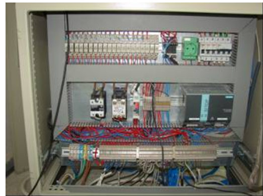
Fig. 12 Control panel
