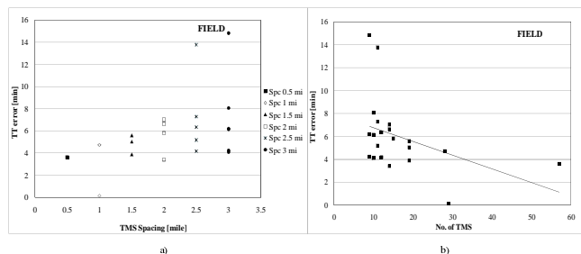
Fig. 4 Field Results (a) Travel time error as a function of TMS spacing (b) Travel time error as a function of number of TMS deployed
