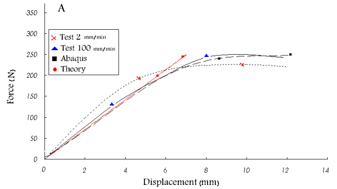
Fig 19 Three point bending in sandwich beam of A
