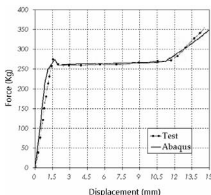
Fig. 2 PVC loading in uniaxial with velocity 2mm/min
