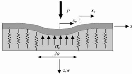
Fig. 11 Indentation model of sandwich beams [9]
