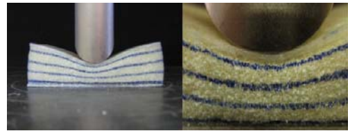
Fig 12 Indentation in sandwich beam with PU core
