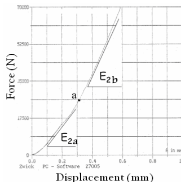
Fig. 3 Lateral compression in 4layer composite laminate
